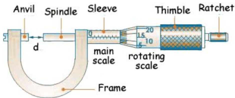
Figure 1.3 micrometer screw gauge
