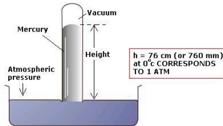
Figure 5.12 diagram of a simple mercury barometer.
