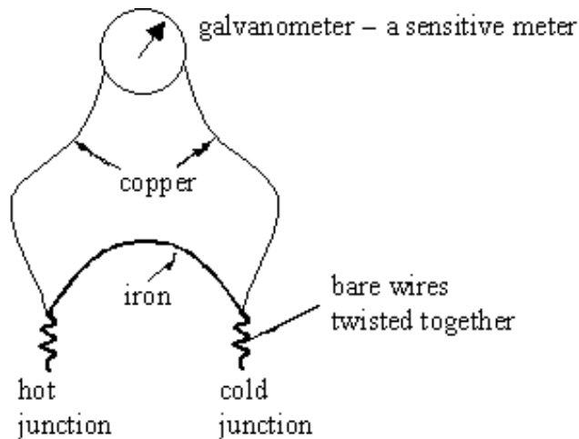
Figure 4.3: thermocouple
