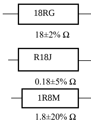
Figure 11.23 resistance code standard notation
