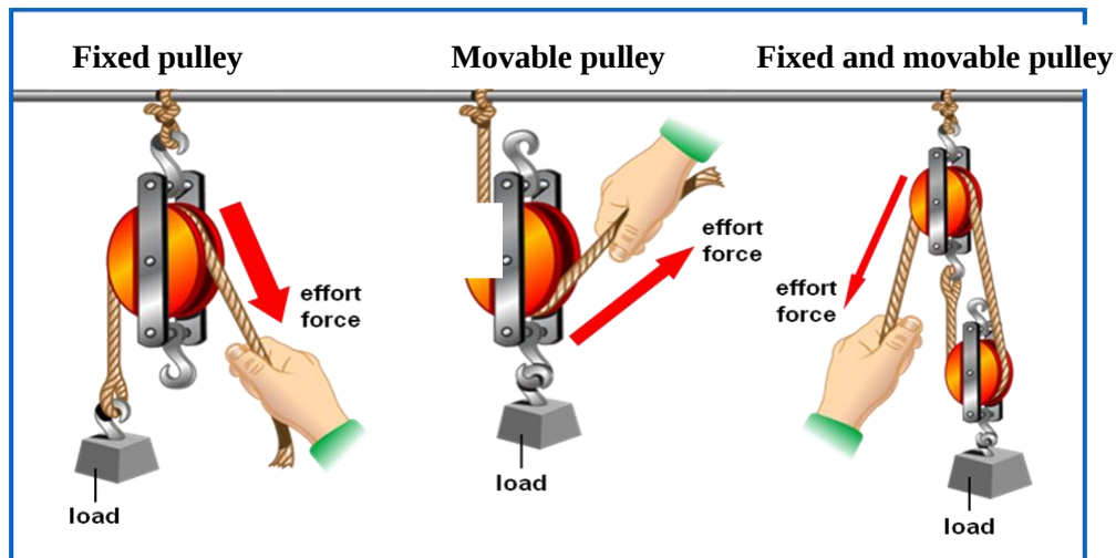
Figure 9.2 pulley systems
