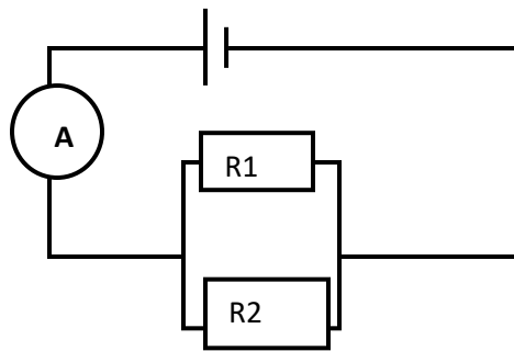
Figure 11.27 parallel circuit
