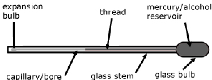
Figure 4.1: a liquid-in-glass thermometer
