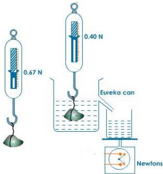
Figure 5.16 apparent weight
