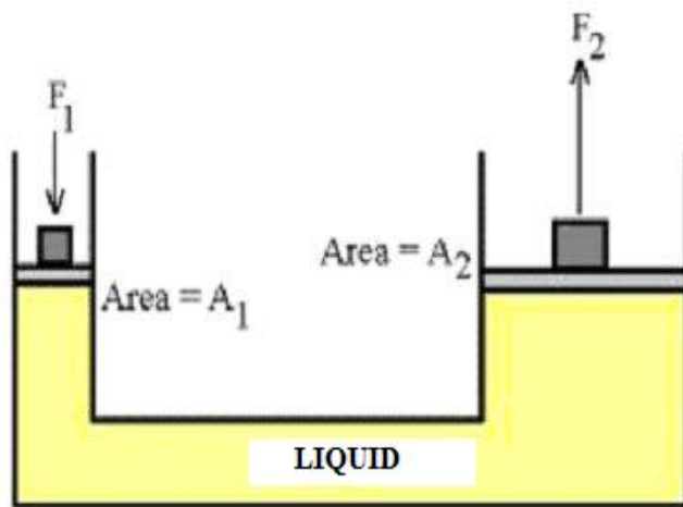
Figure 5.14 hydraulic machine.
