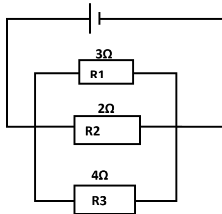
Figure 11.35 resistors connected in parallel
