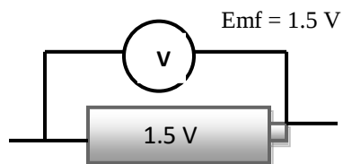
Figure 11.5 measuring Emf
