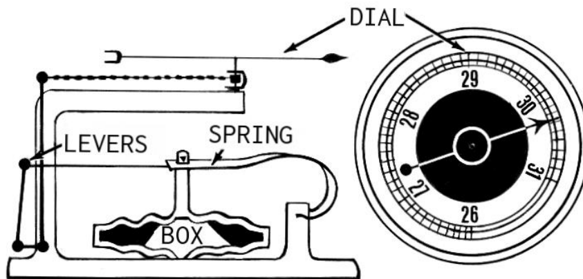
Figure 5.13 aneroid barometer
