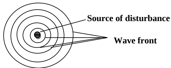
Figure 12.14 circular wave front
