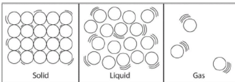
Figure 3.1 arrangement of particles in the three states of matter
