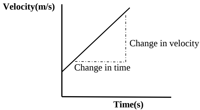
Figure 8.2 graph of velocity against time
