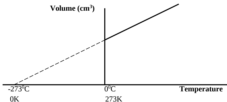
Figure 3.10 Volume of a gas against temperature
