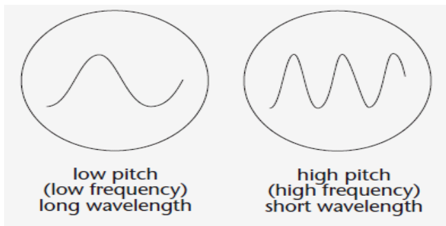
Figure 13.2 effect of frequency on the pitch of sound
