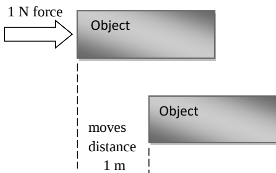
Figure 9.1 demonstrating work done
