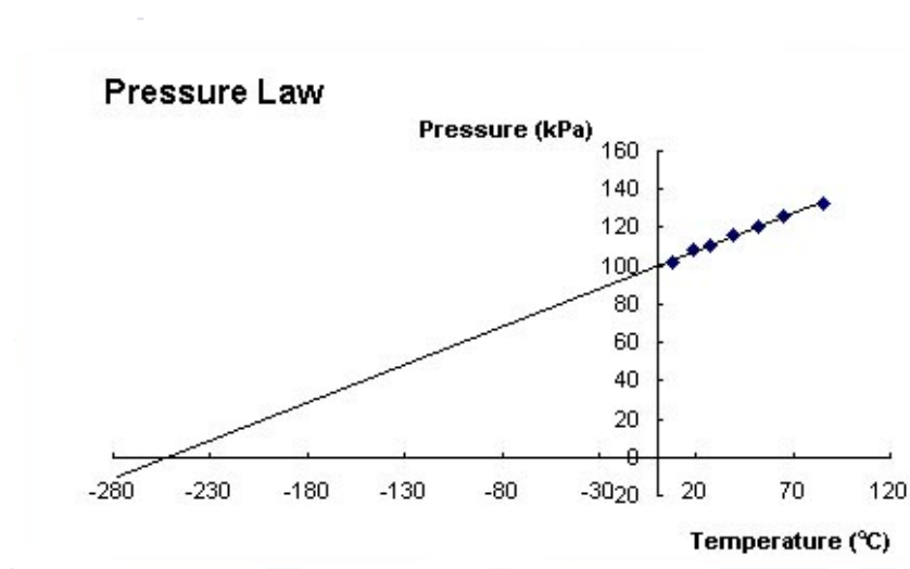
Figure 6.8 graph of pressure of the gas against temperature
