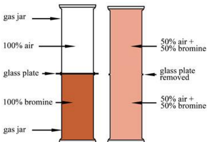
Figure 3.9: diffusion of bromine gas and air
