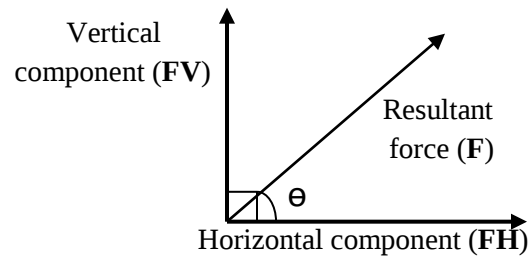
Figure 7.13 components at right angle.
