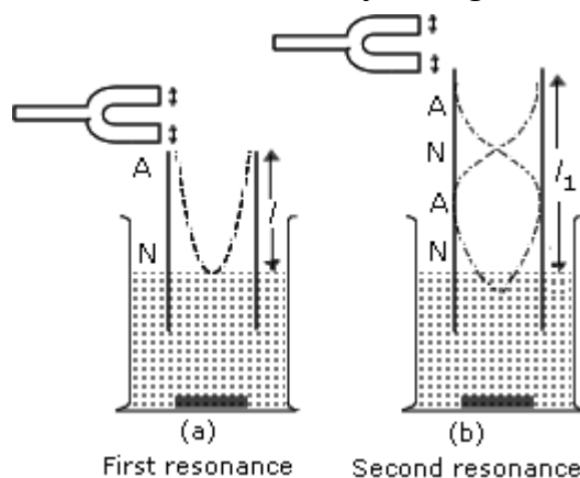
Figure 13.7 Resonance in a jar with water
