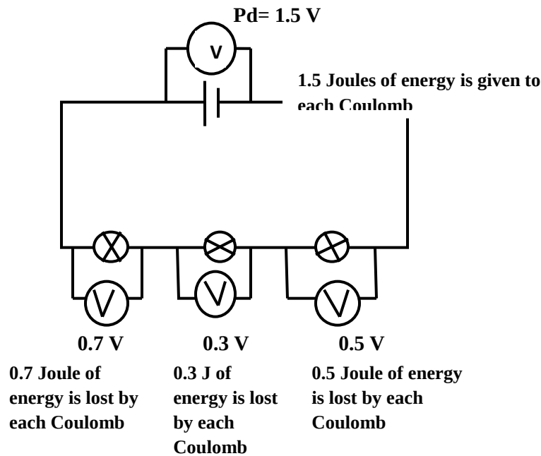
Figure 11.4 Measuring potential difference using a voltmeter
