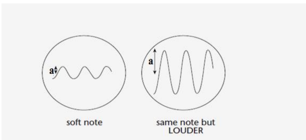
Figure 13.1 effect of amplitude of the wave on loudness of sound
