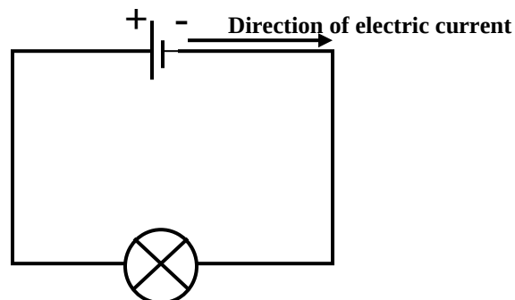
Figure 11.1 direction of electric current
