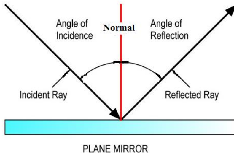
Figure 12.22 Reflection in a light wave
