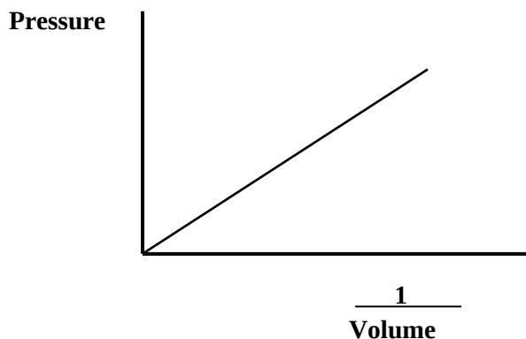
Figure 6.4 pressure is directly proportional to 1/volume
