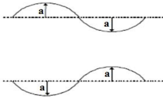
Figure 12.13 (b) the waves are out of phase
