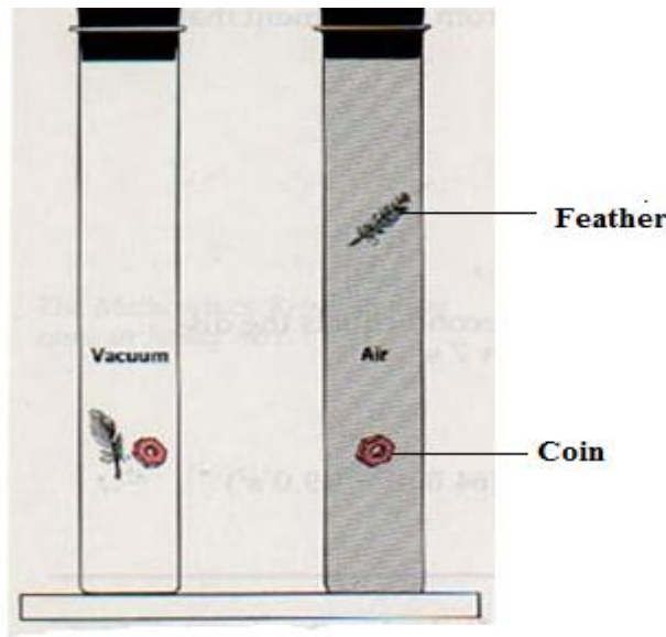
Figure 8.14 falling in a vacuum and air
