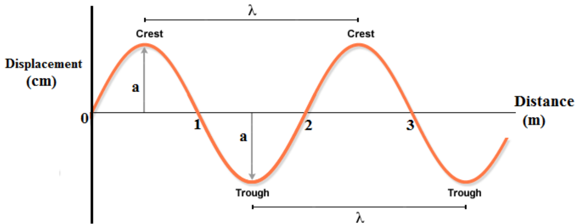
Figure 12.11 showing the wave length of the wave
