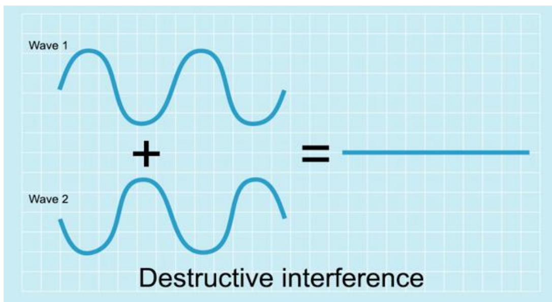
Figure 12.29 destructive interference
