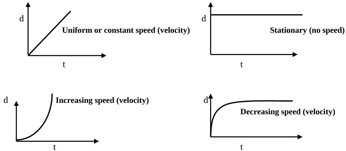
Figure 8.5 distance (displacement) – time graphs
