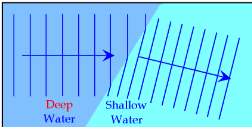
Figure 12.23 Refraction of a water wave.
