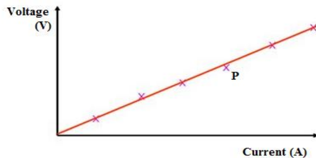
Figure 2.7 line of best fit
