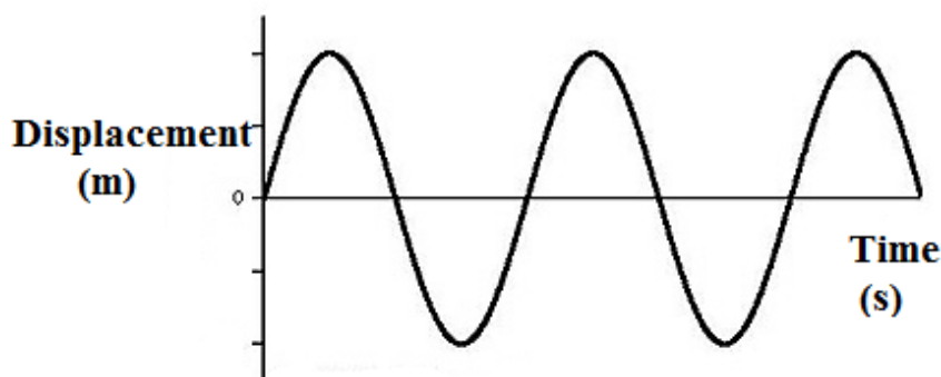
Figure 12.8 A wave
