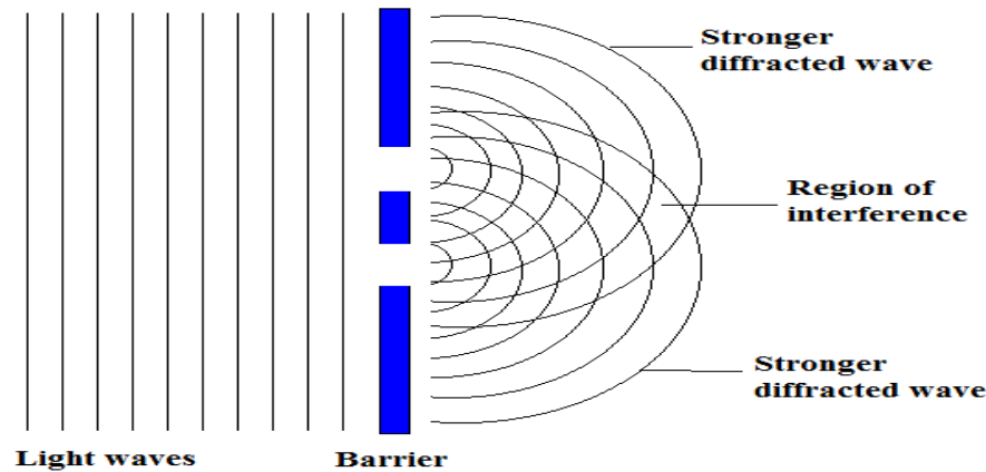
Figure 12.27 Diffraction of a wave in two slits
