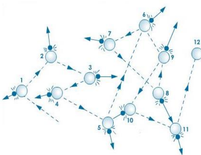
Figure 3.8 Brownian motion of gas molecules.
