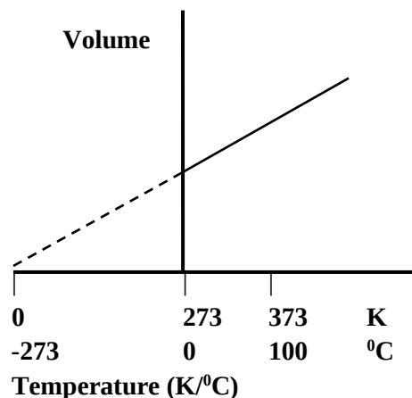
Figure 6.6 graph of volume against temperature
