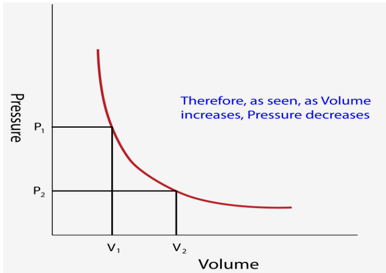
Figure 6.2 graph of pressure of the gas against volume
