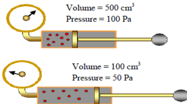
Figure 6.3 relationship between volume and pressure
