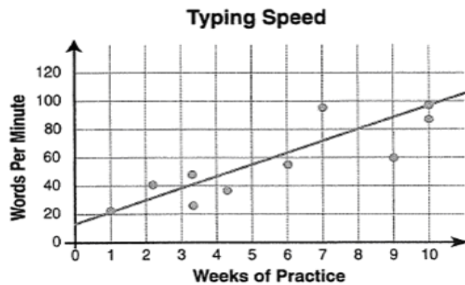
Figure 2.8 graph of best fit
