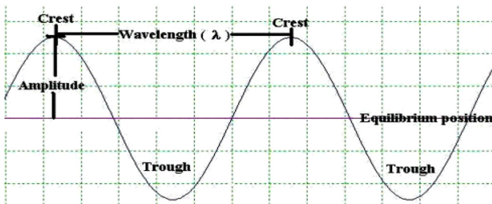
Figure 12.20 a transverse wave
