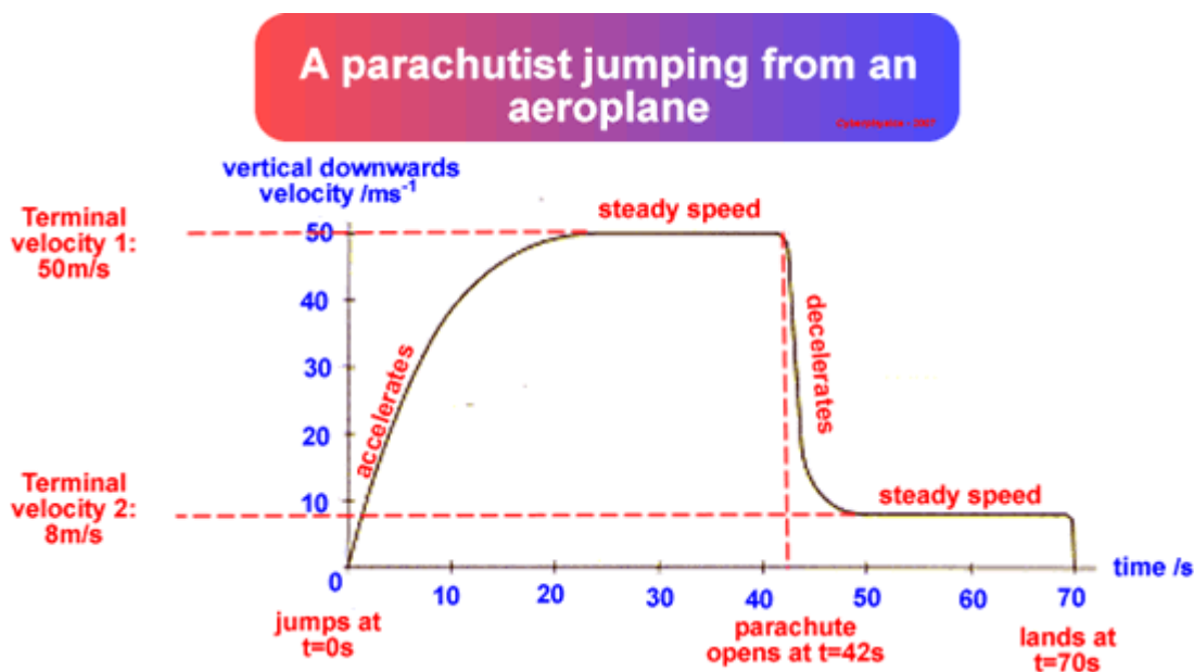
Figure 8.16 graph of a parachutist.
