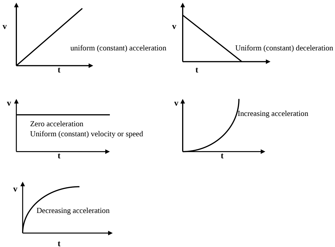
Figure 8.8 velocity- time graphs
