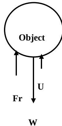
Figure 8.12 forces acting on a falling object
