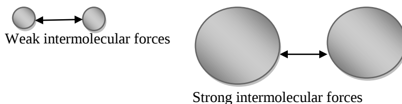
Figure 3.3 effect of size of the particles on intermolecular forces
