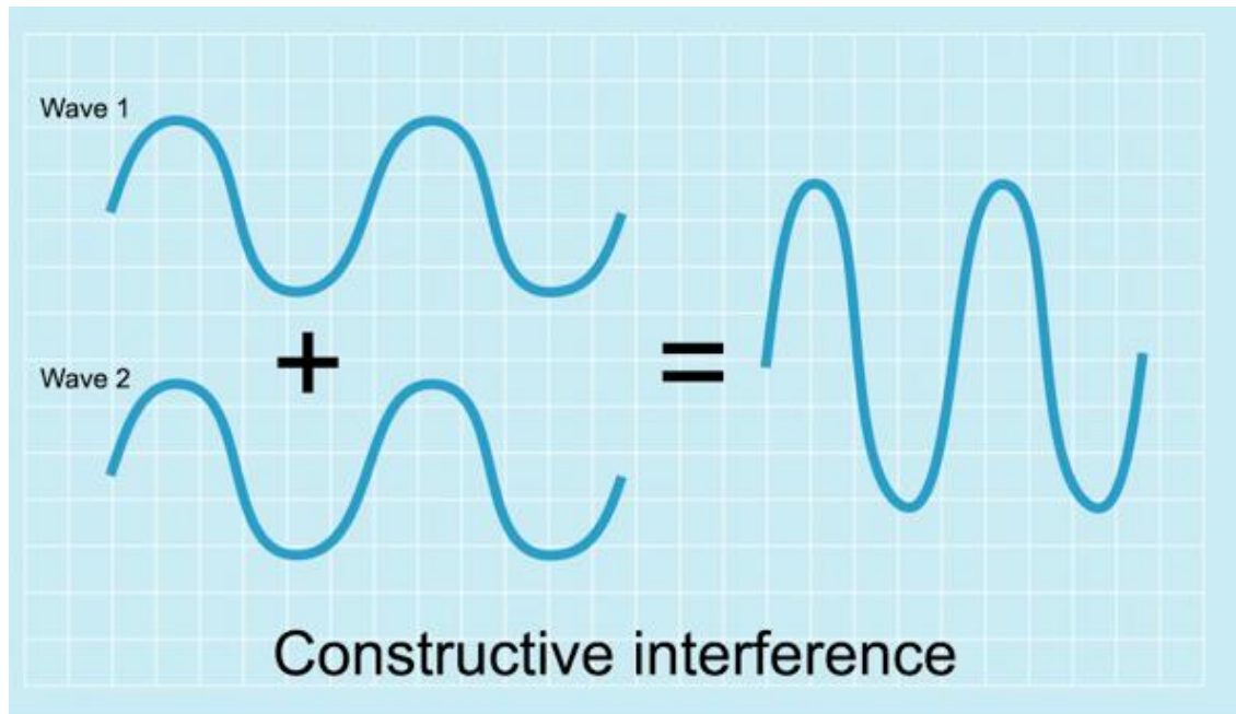
Figure 12.28 constructive interference
