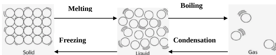
Figure 3.7 changes of states of matter
