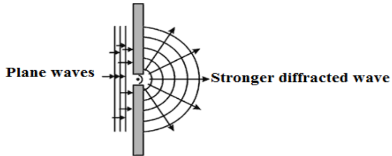
Figure 12.25 diffraction of a wave in a narrow gap
