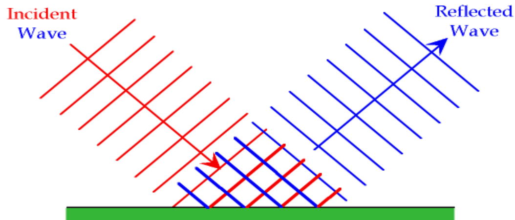
Figure 12.21 Reflection in a water wave
