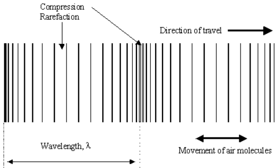
Figure 12.18 longitudinal wave
