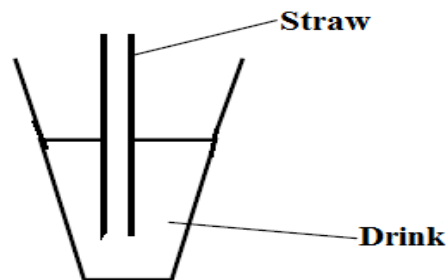
Figure 5.9 drinking through a straw
