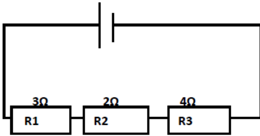
Figure 11.34 resistors connected in series.
