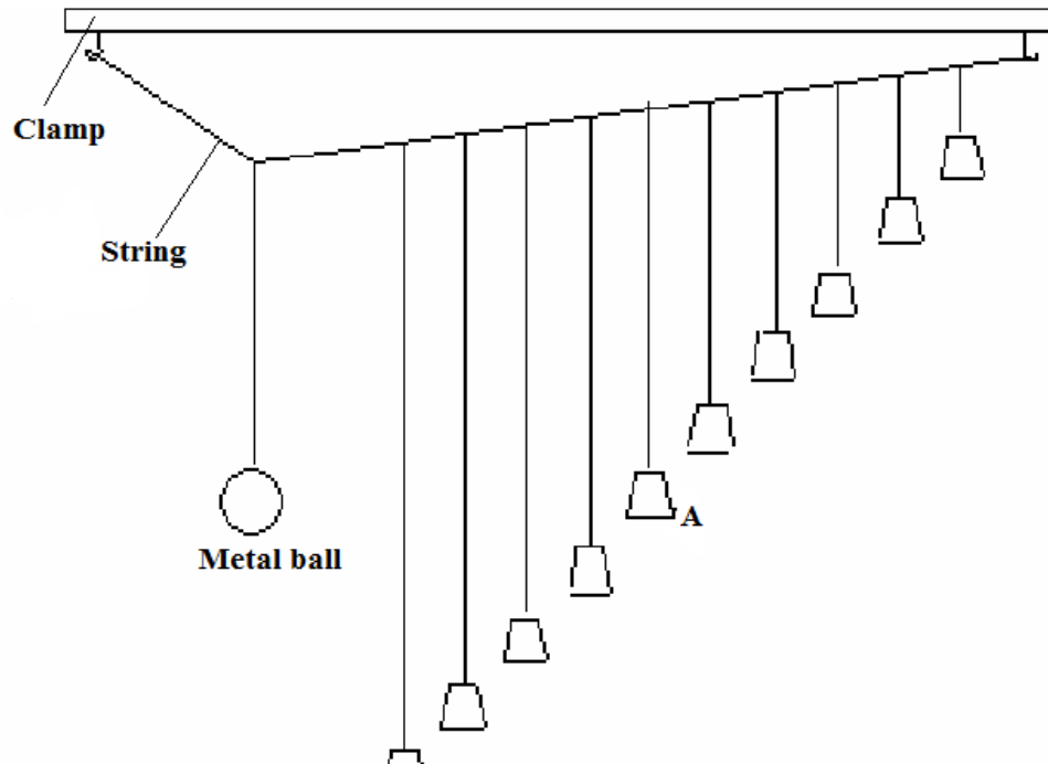
Figure 13.5 Barton's pendulum
