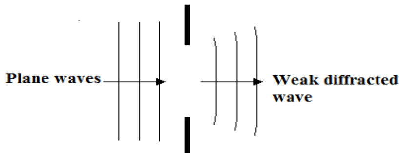
Figure 12.26 diffraction of a wave in a wide gap
