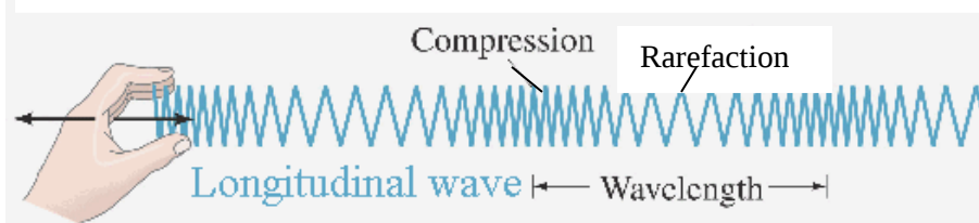
Figure 12.17 demonstrating longitudinal wave in a spring
