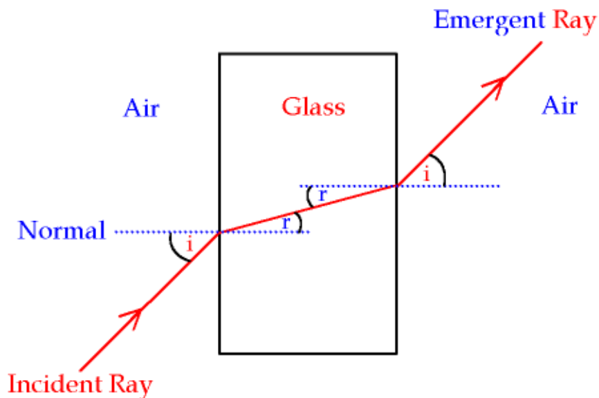
Figure 12.24 Refraction of a light wave
