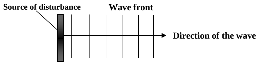
Figure 12.15 straight wave front
