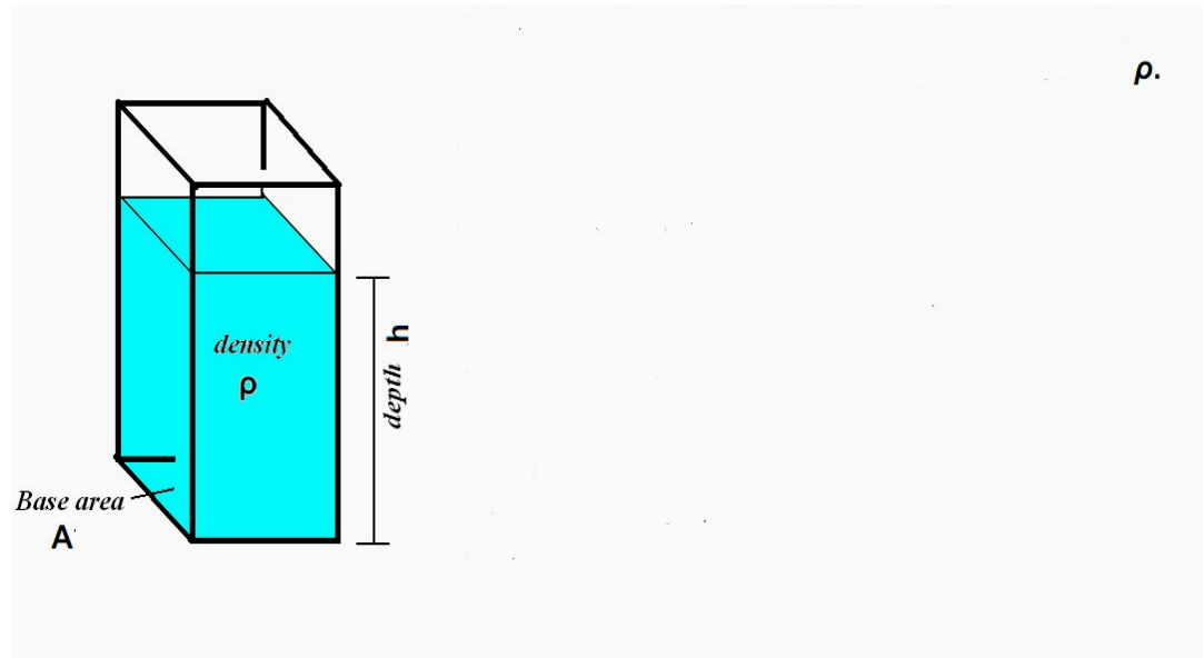
Figure 5 .6 Pressure in liquid
