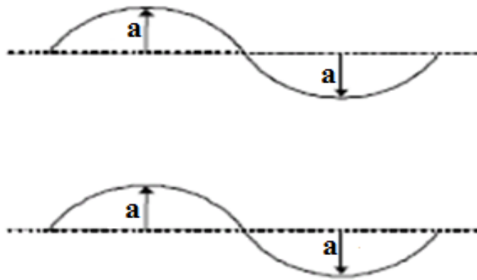
Figure 12.13(a) the waves are in phase
