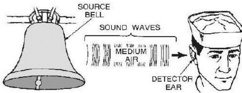
Figure 13.9 transmission of sound in air
