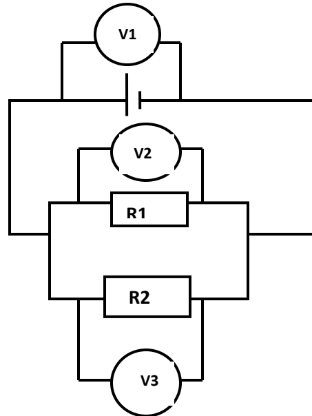
Figure 11.33 voltages in parallel circuit.
