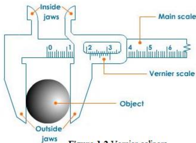
Figure 1.2 Vernier calipers
