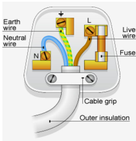
Figure 11.47 three-pin plug
