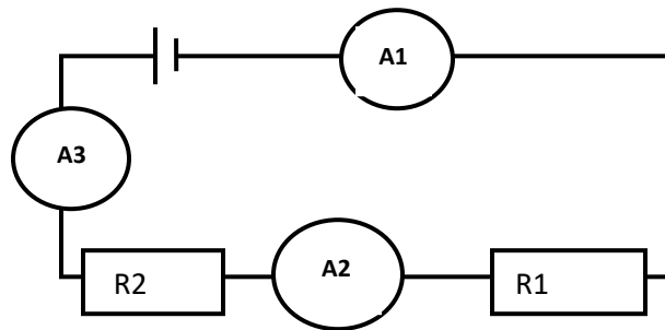
Figure 11.30 current flowing in series circuit
