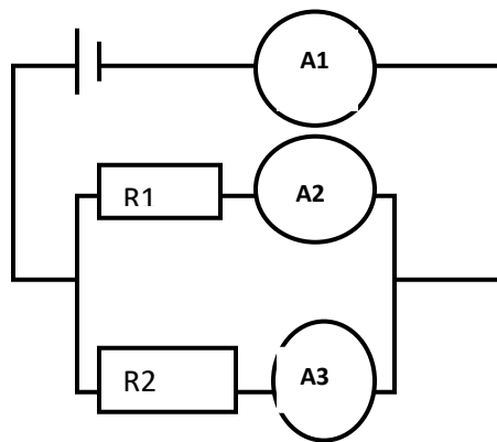
Figure 11.31 current flowing in a parallel circuit.
